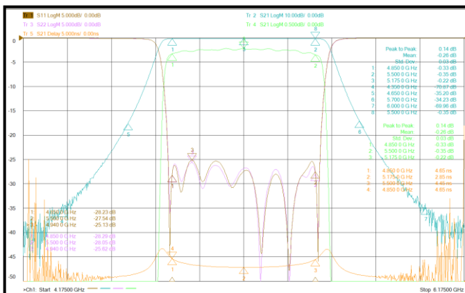
< Insertion Loss / Return Loss measurement >
